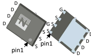
DFN5*6
